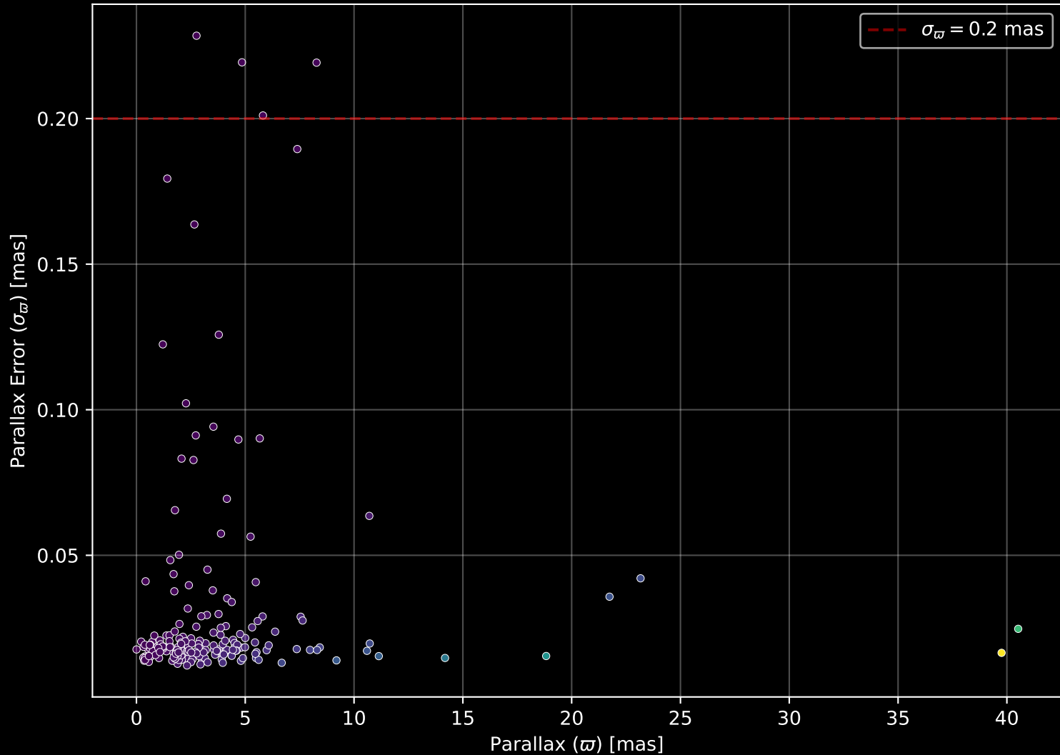
APOGEE DR17 Field: [090-42_MGA] Parallax Quality (n= 198)
