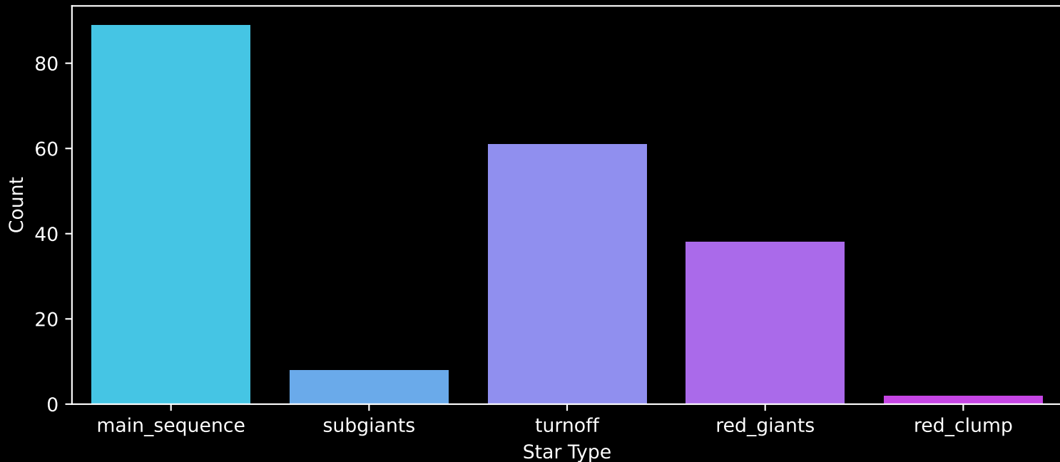
APOGEE DR17 Field: [090-42_MGA] Count plot of Star Type
