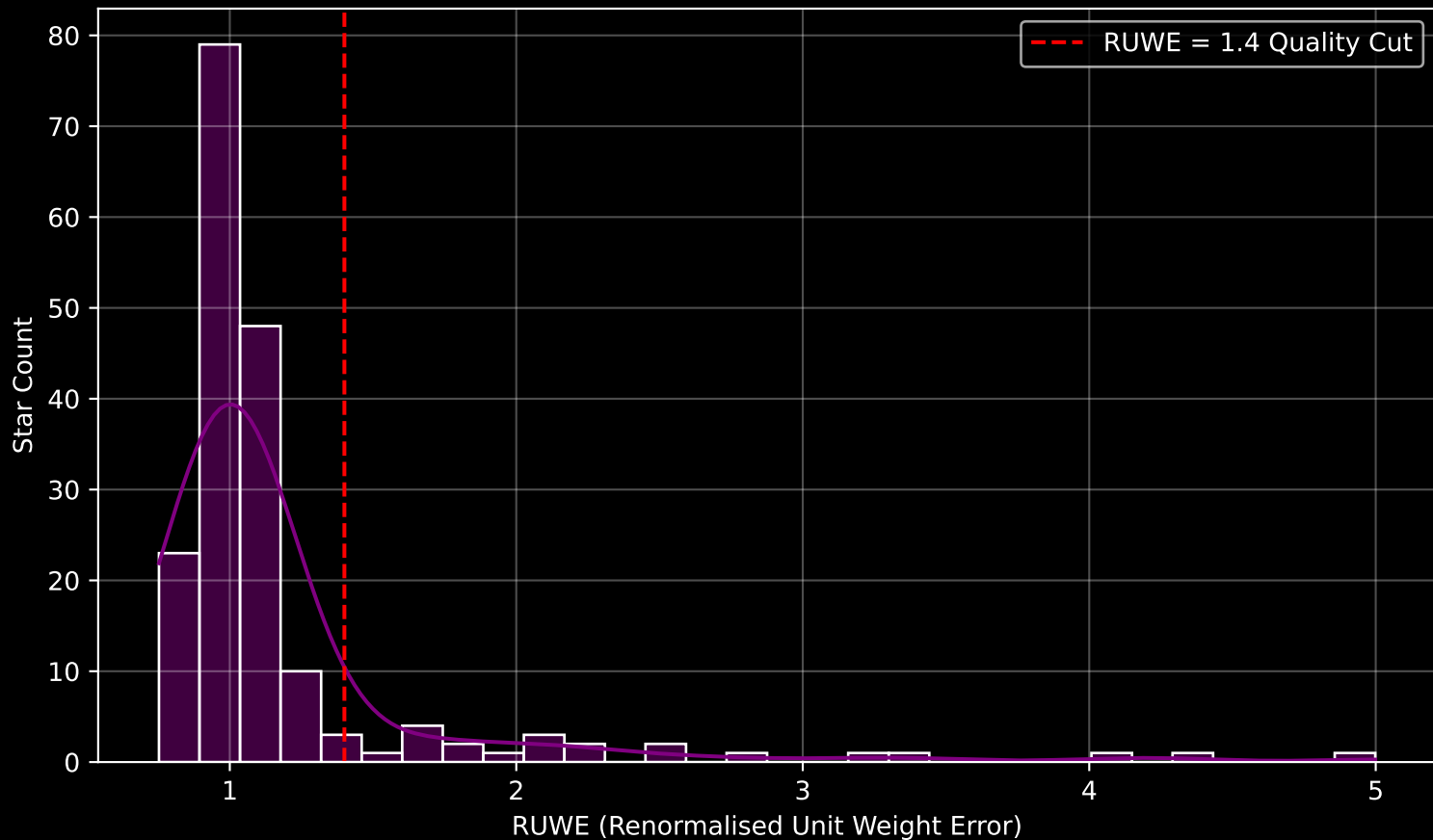
GAPOGEE DR17 Field [090-42_MGA] RUWE Distribution (n= 184)
