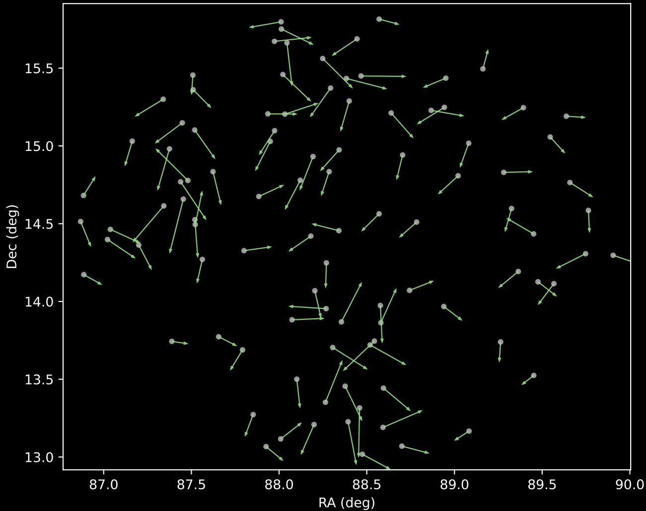
APOGEE DR17 Cluster 5 Proper Motion Vectors (n=99)
