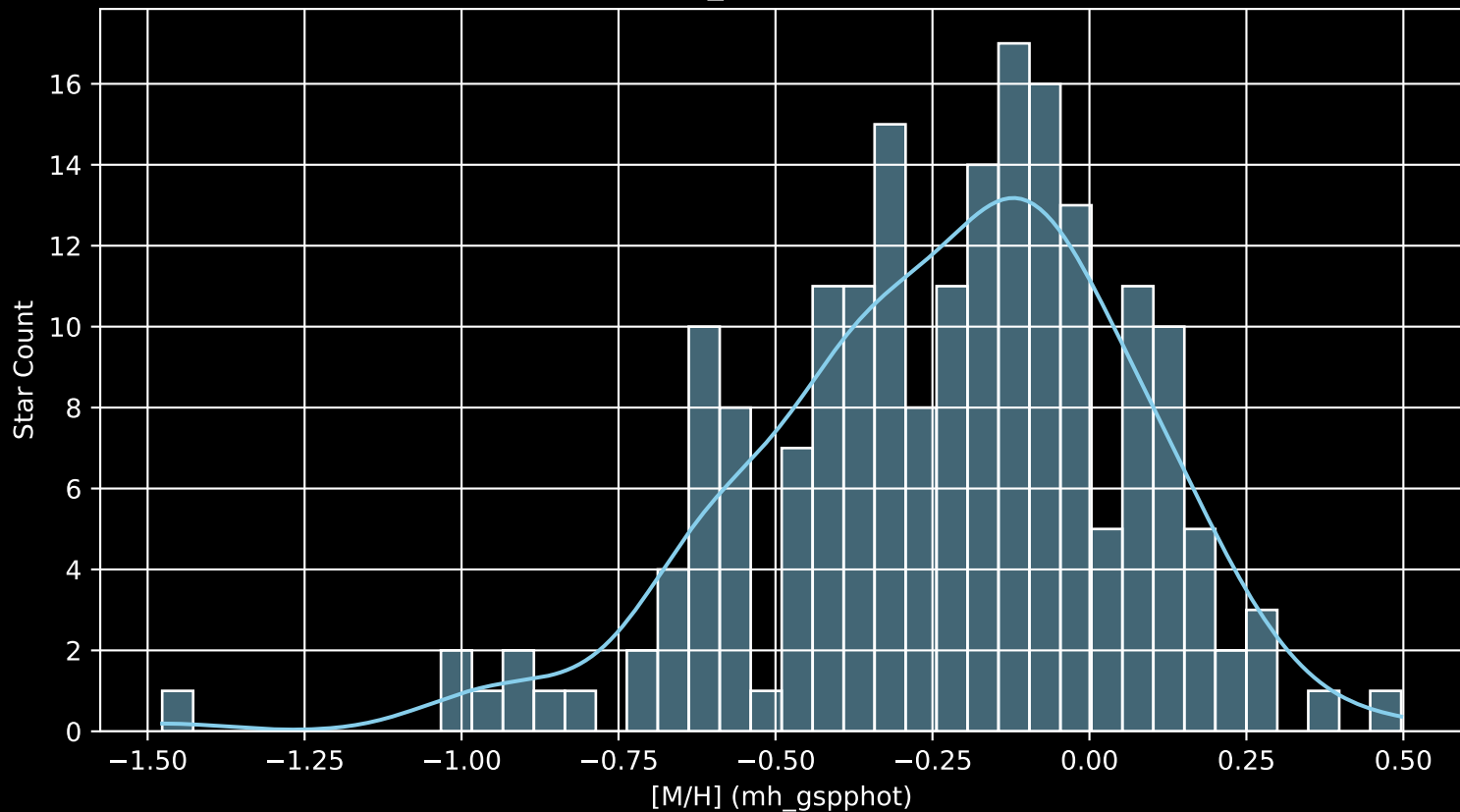
APOGEE DR17 Field: [090-42_MGA [M/H] (mh_gspphot) (n= 194)
