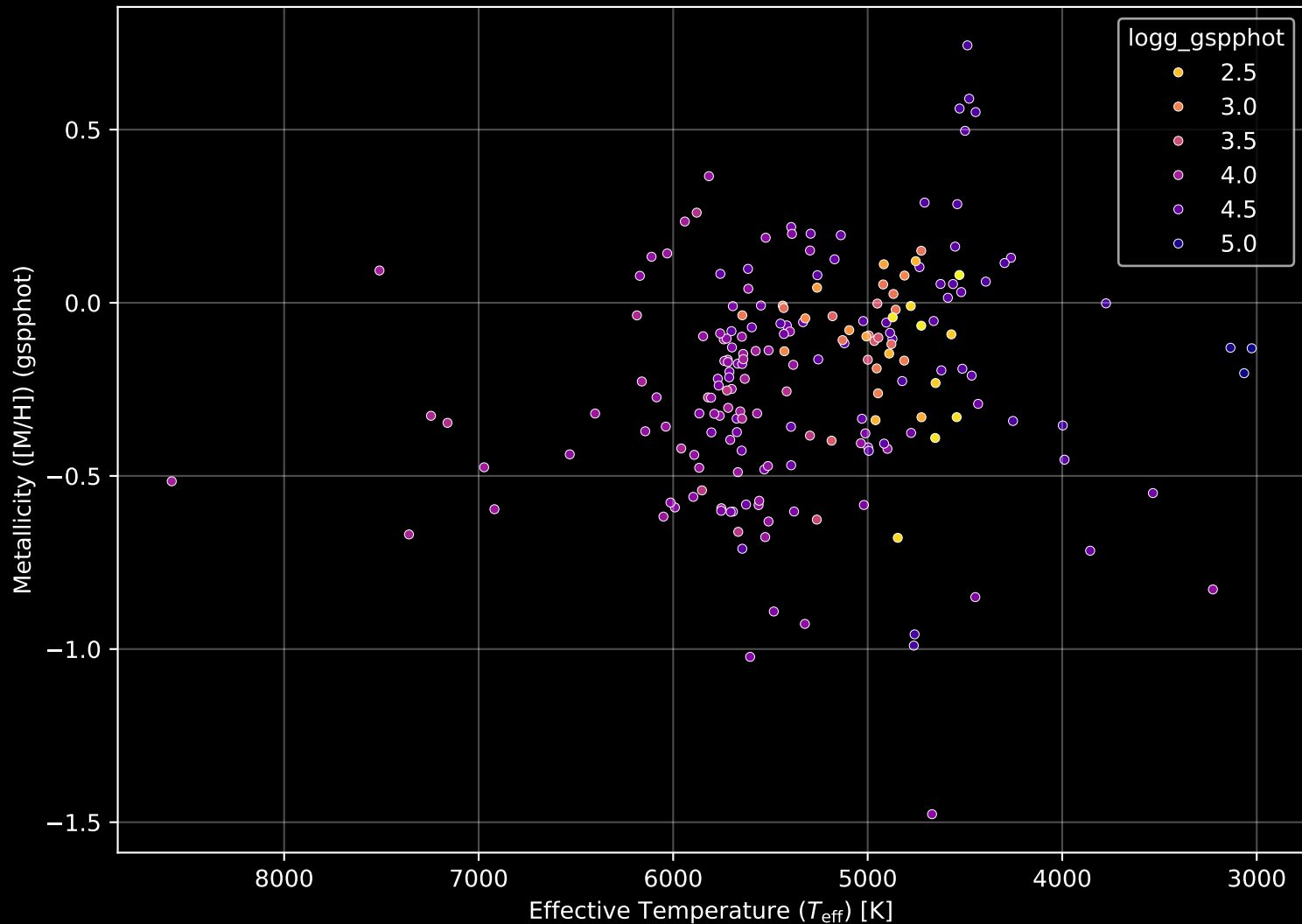
APOGEE DR17 Field: [090-42_MGA] Stellar Population Parameters (n= 198)
