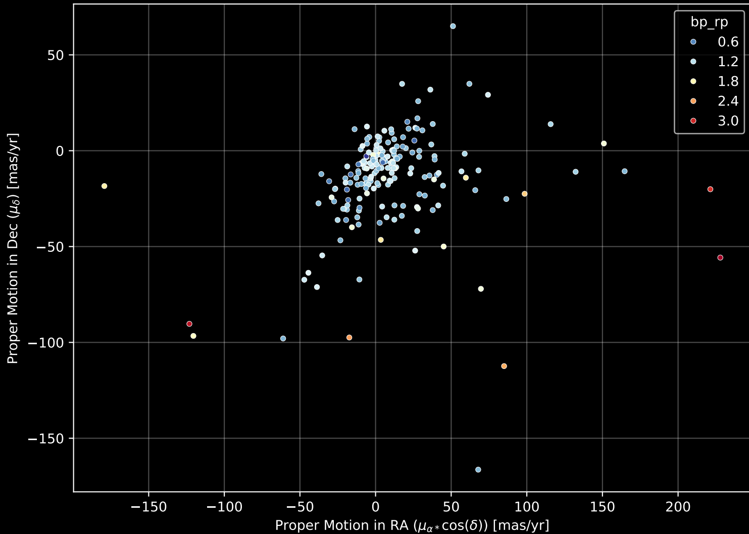
APOGEE DR17 Field: [090-42_MGA] Proper Motion Diagram (n= 198)
